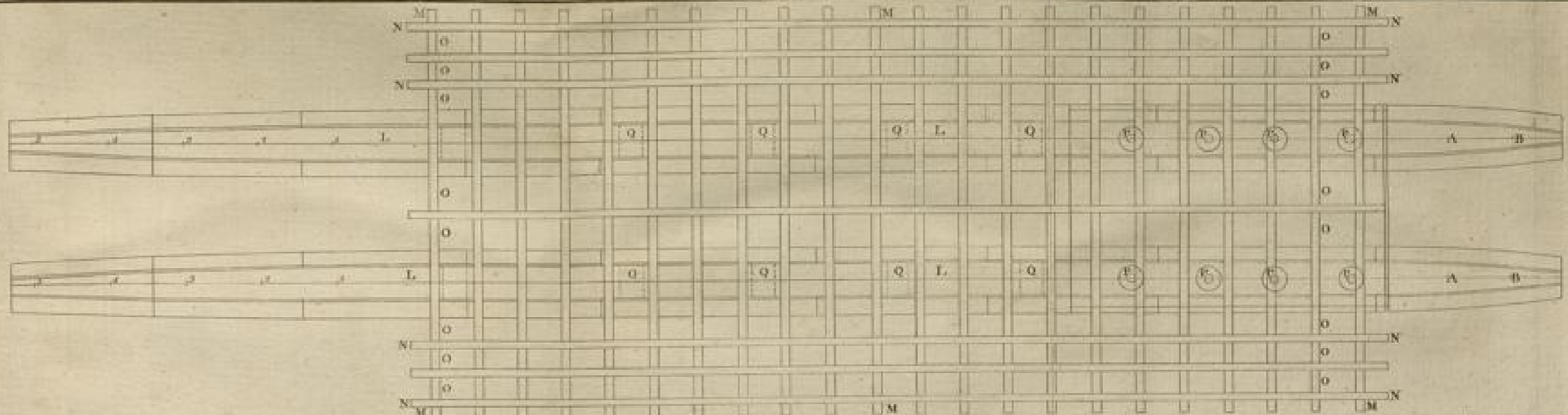
A Draught Plan and Section of the Britannia Ocheite War Cannon, showing Two in the Plan, the Distance being from out to Outside 14' 3" and secured with Beams and Fore and Aft Pieces of Timber lashed together with Sinnet made of Cocoa Nut Buds.
