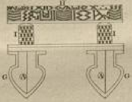
A Draught Plan and Section of the Britannia Ocheite War Cannon, showing Two in the Plan, the Distance being from out to Outside 14' 3" and secured with Beams and Fore and Aft Pieces of Timber lashed together with Sinnet made of Cocoa Nut Buds.
